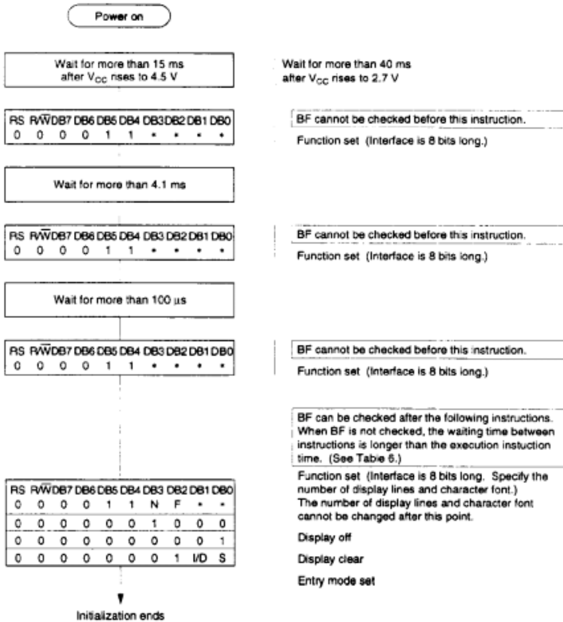
Figure 5: 8 Bit Interface
