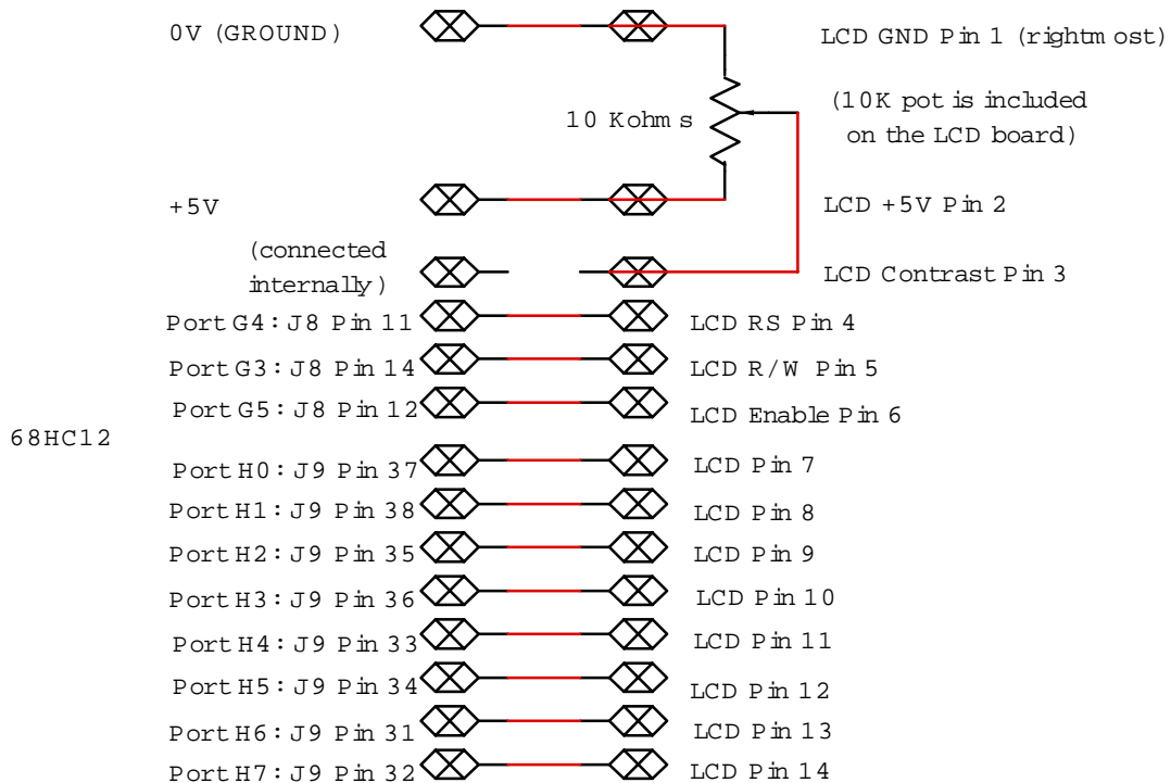
68HC12 LCD Wiring Connections
