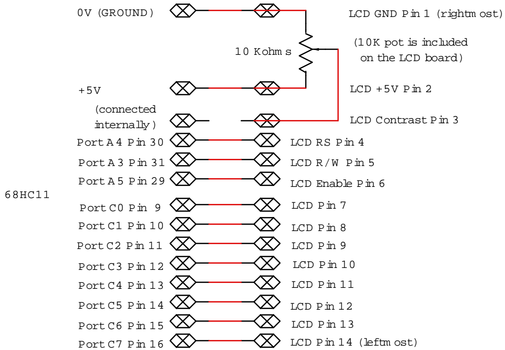
68HC11 LCD Wiring Connections
