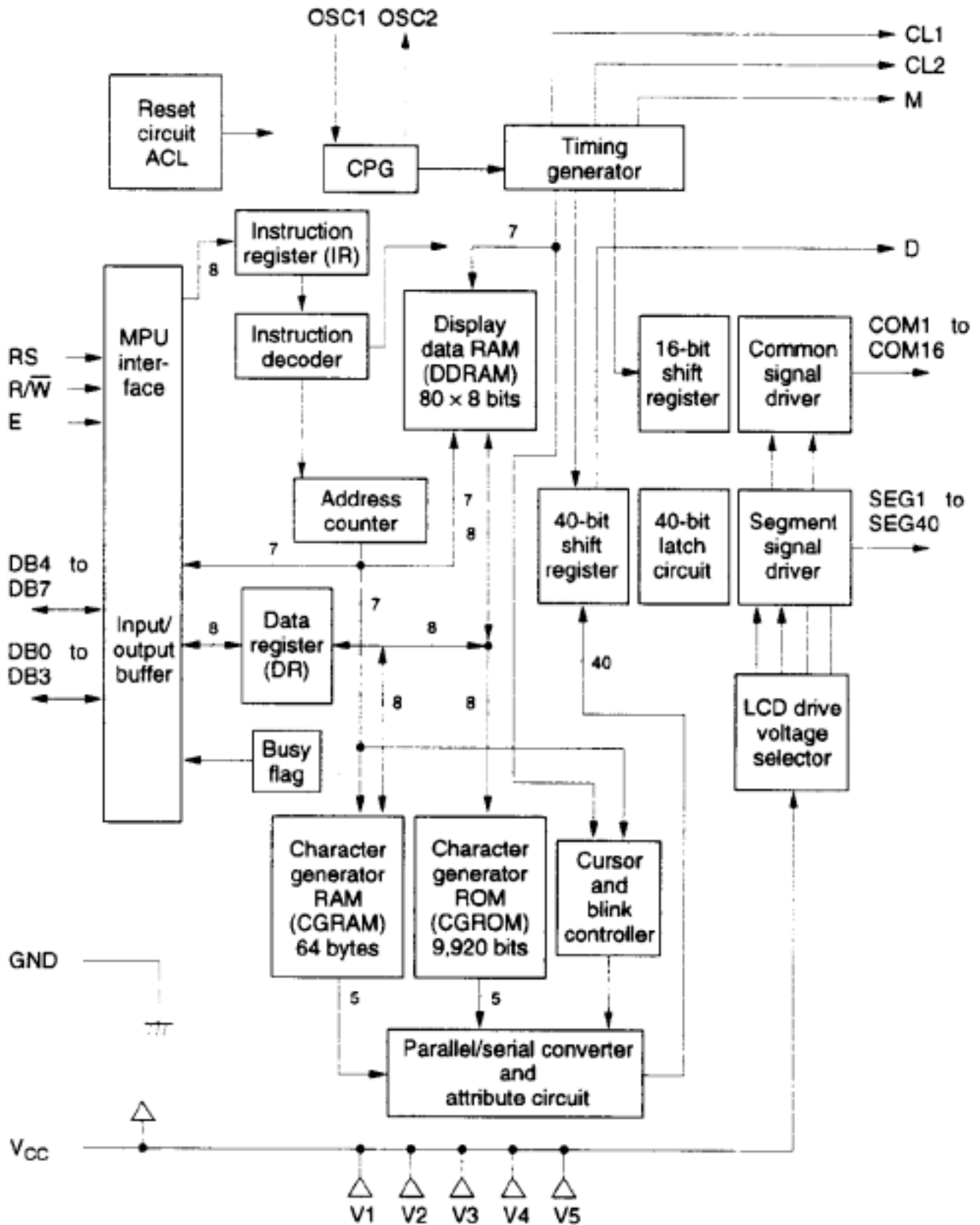
Figure 1: HD44780U Block Diagram
